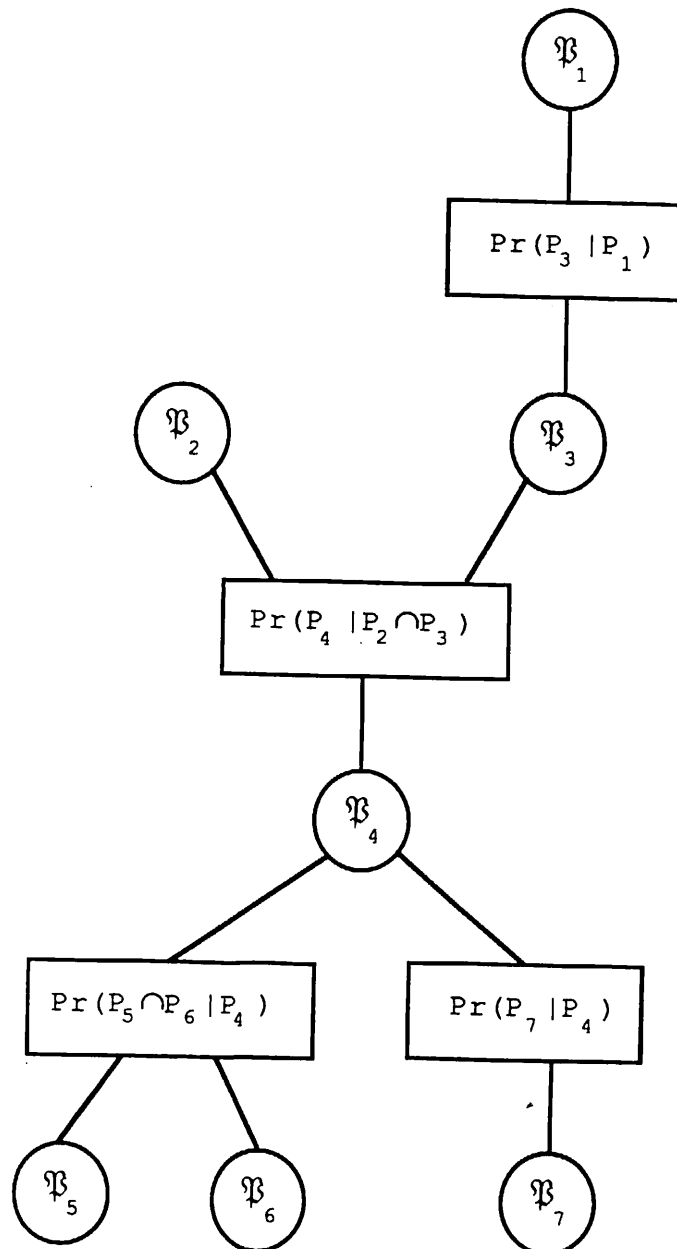
Figure 11. General Bayesian Propagation
