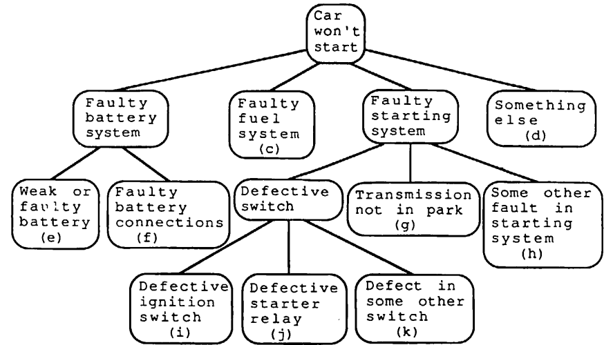
Figure 2. A Tree of Diagnoses
