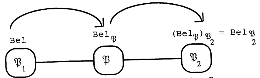
Figure 7. Projecting a Belief Function From \mathfrak{B}_1 to \mathfrak{B}_2
