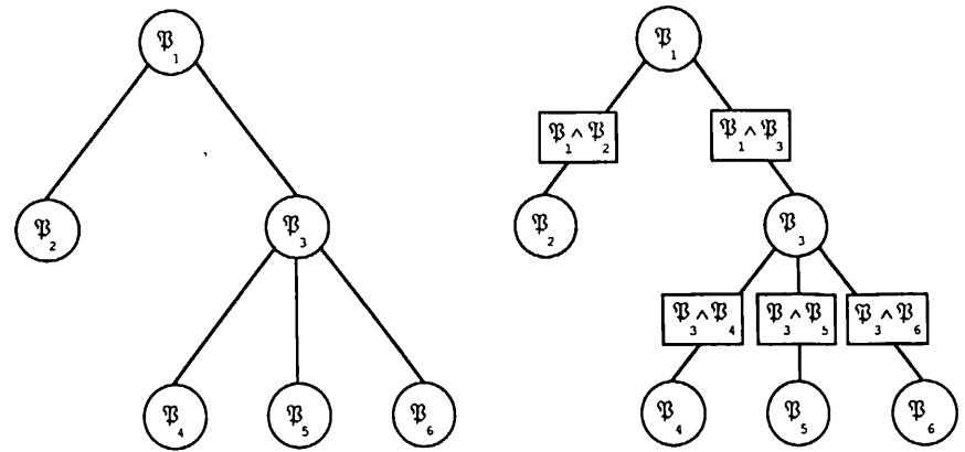
Figure 10. Interpolation in a Rooted Markov Tree
