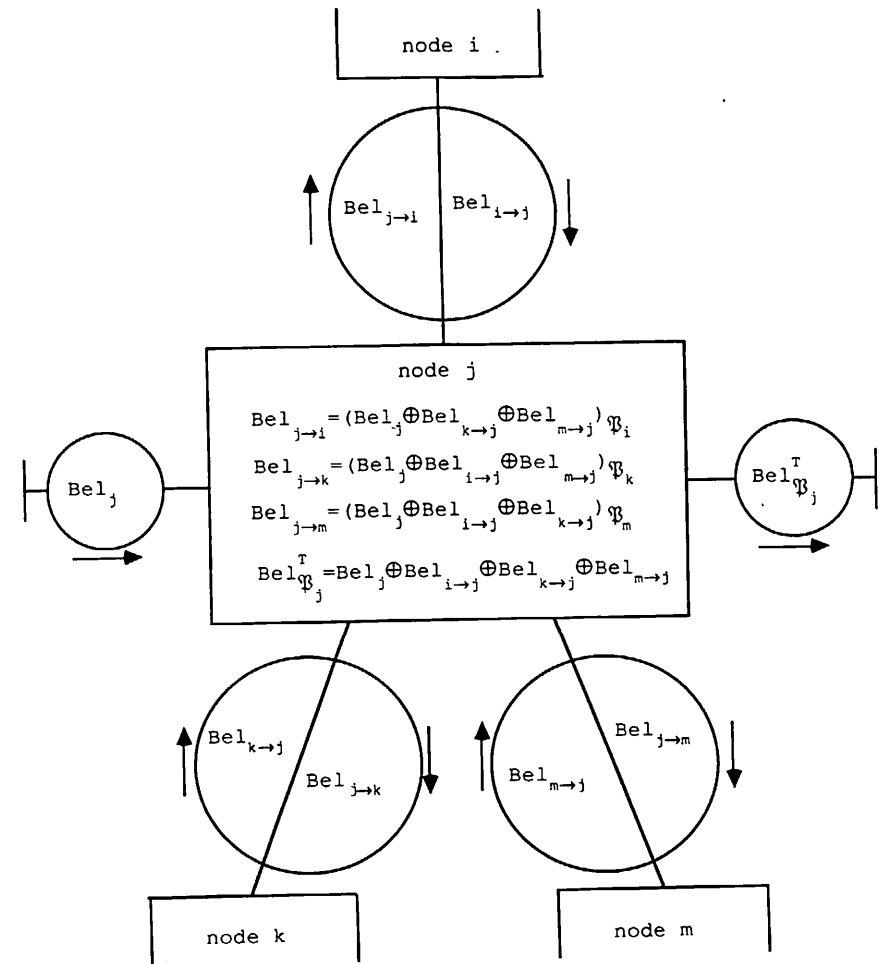
Figure 9. A Typical Processor (with Three Neighbors)
