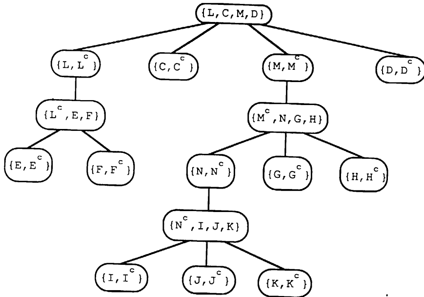
Figure 5. The Tree of Families and Dichotomies
